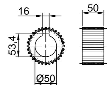
PINION
