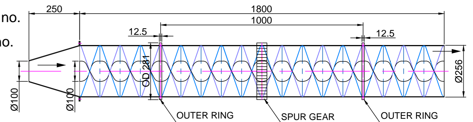
ASSEMBLY OF SCREW CONVEYOR
