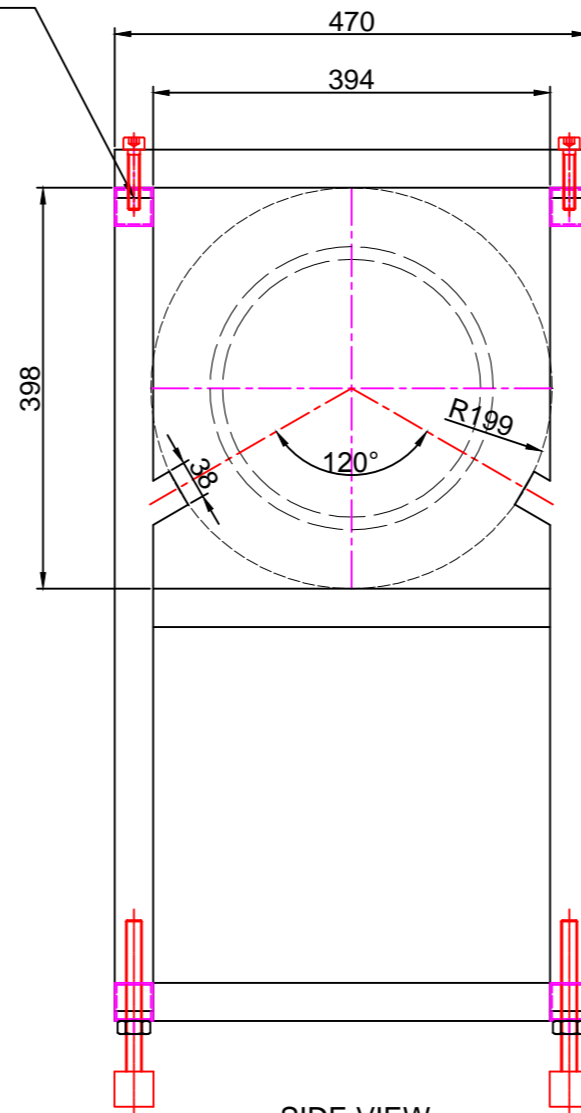
SIDE VIEW
