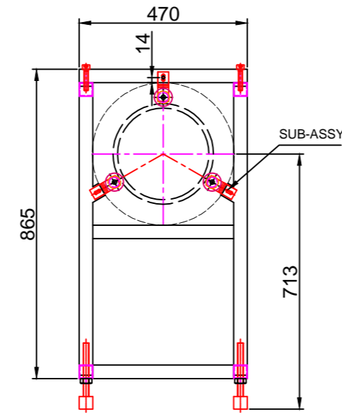
ASSEMBLY WITH ROLLER - SIDE VIEW
