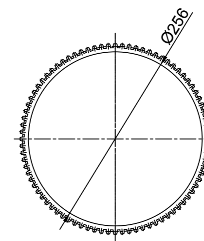
SPUR GEAR
