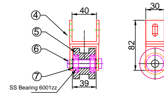
SUB - ASSEMBLY (ROLLER)
