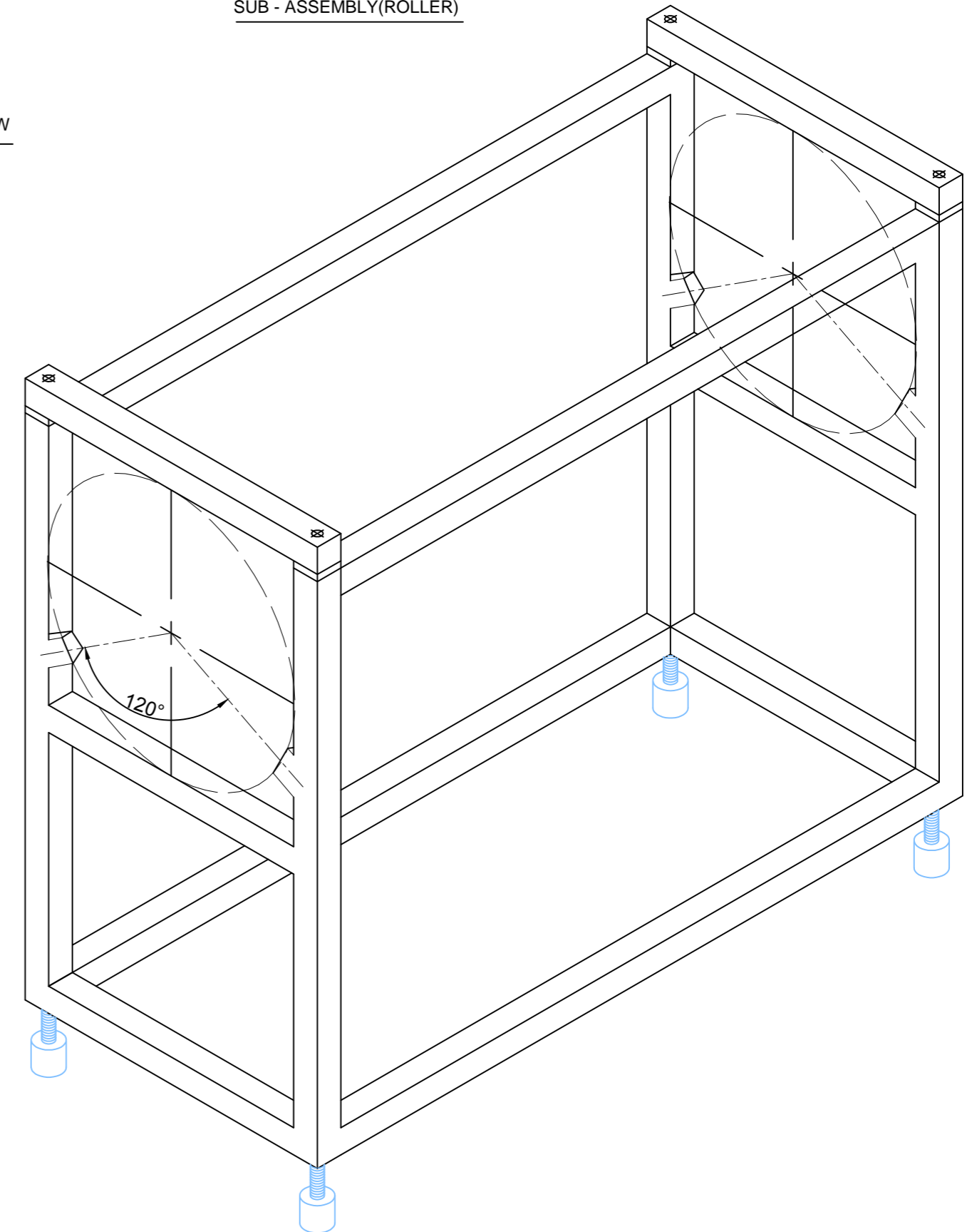
SUB - ASSEMBLY (ROLLER)
