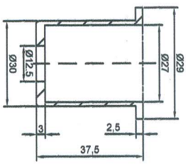
④ SPRING HOLDER Matlle:- NYLON 66 Grade vigin Qty:- 1No.
