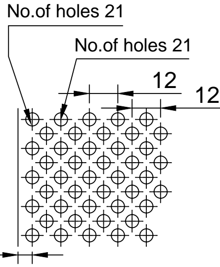
Partial development of PVC core Ø80x780 L
