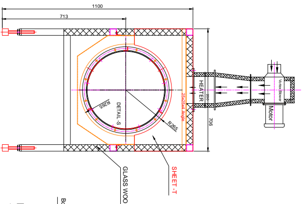
HEATING BOOTH BOTTOM SHEET
