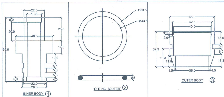
ASSEMBLY VIEW FOR A&B -TYPE
