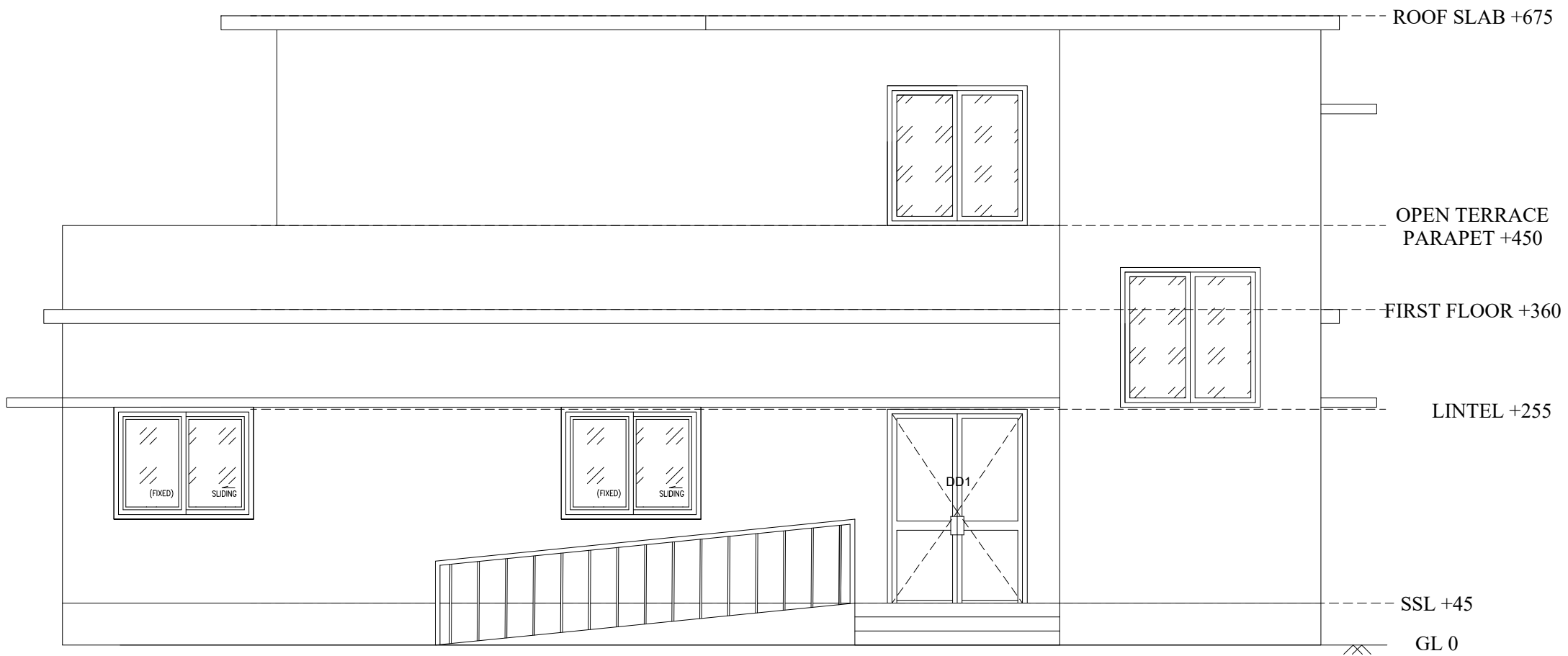
FRONT ELEVATION
