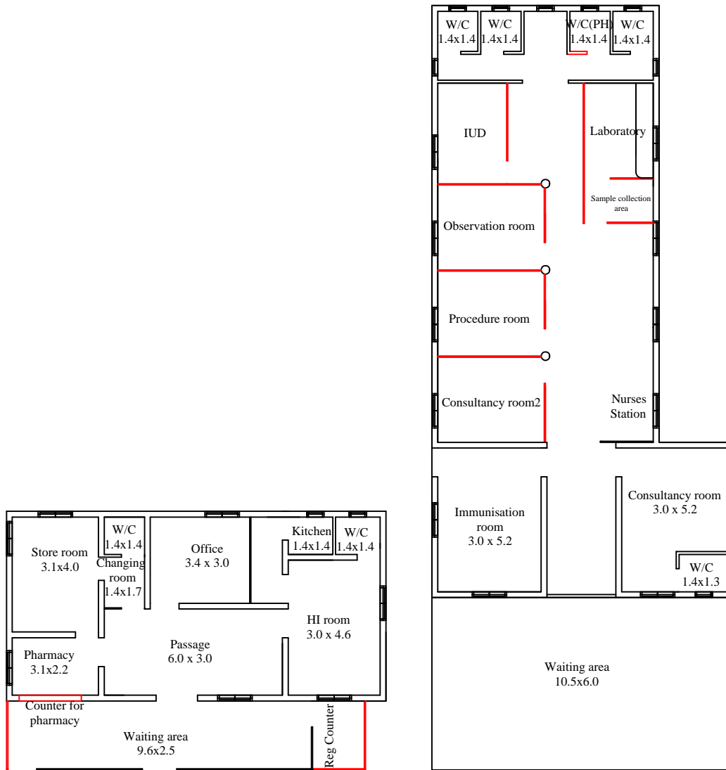
EXISTING OFFICE BLOCK, Area: 110 sqm EXISTING OP BLOCK, Area: 177 sqm
