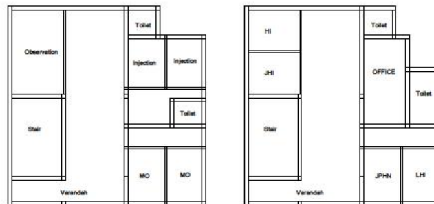
Proposed GF Proposed FF Area of Immunization Building FF:-111.82sqm PRIMARY HEALTH CENTRE TENMALA
