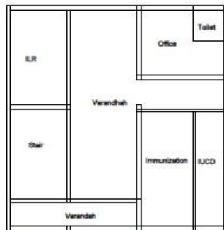
Existing GF
