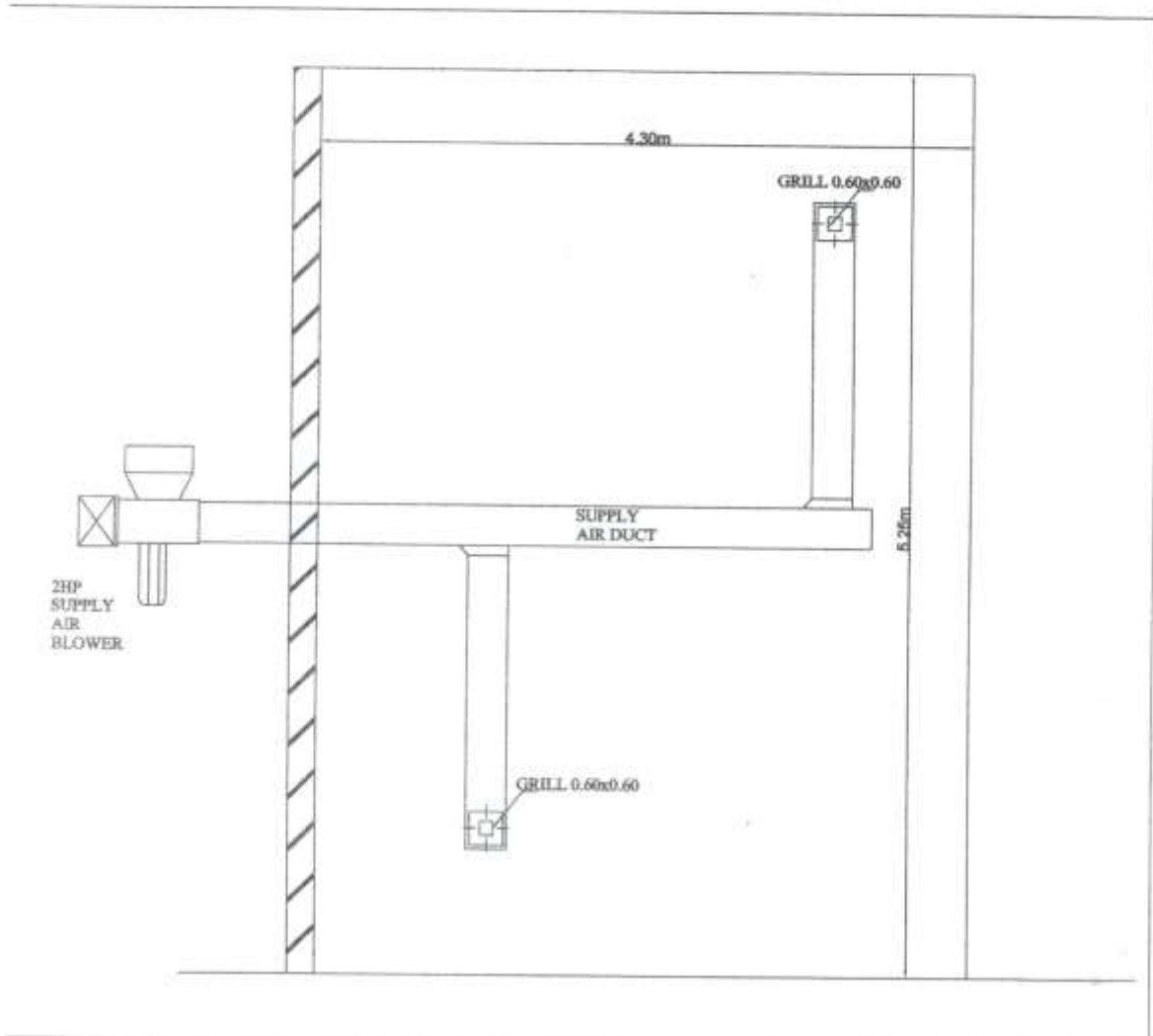
Fresh Air System Plan
