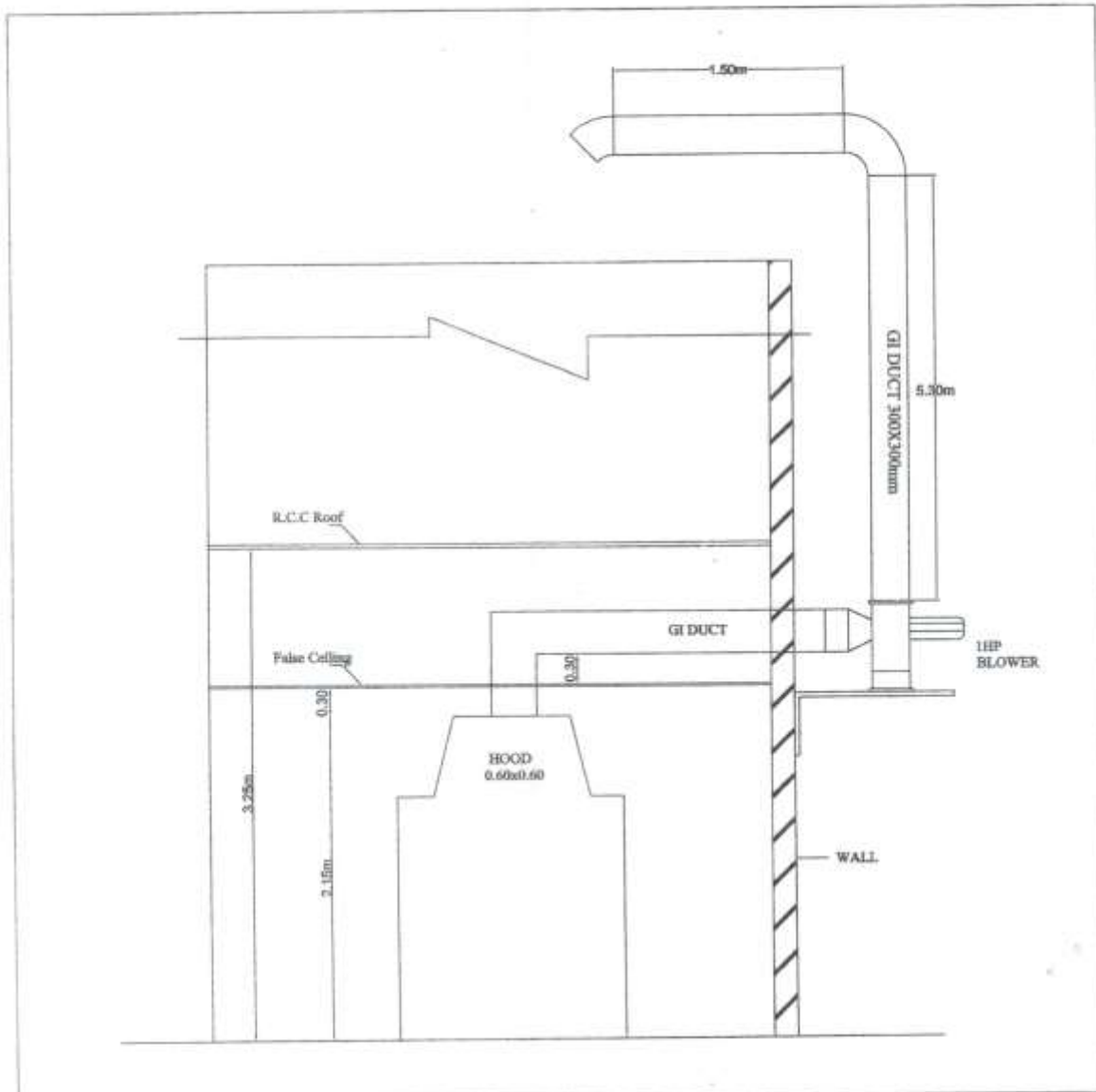
Fume Hood Section
