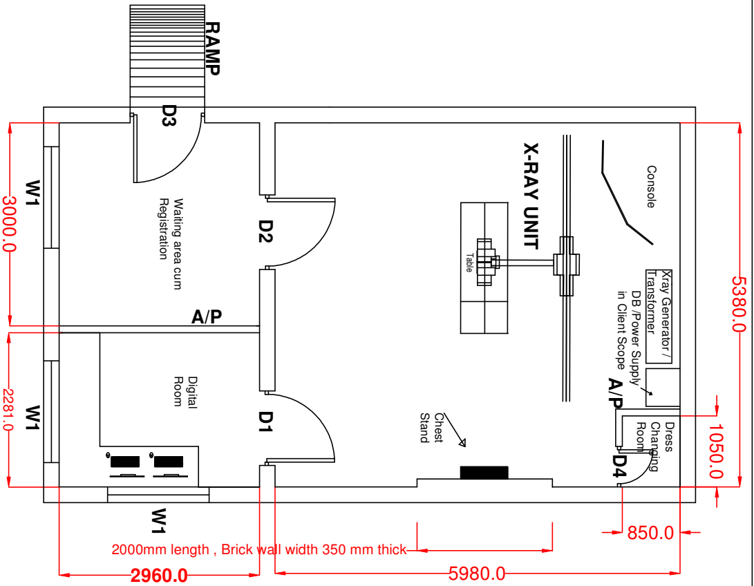
PROPOSED LAYOUT
