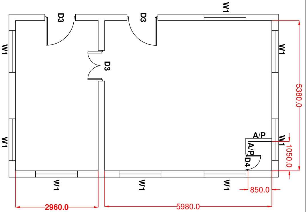
EXISTING LAYOUT
