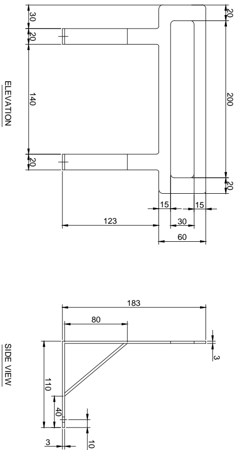
RIGHT SIDE HOLDER
