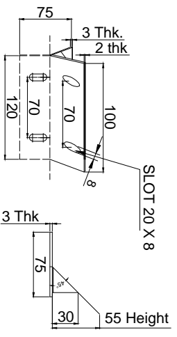
DETAIL - A
